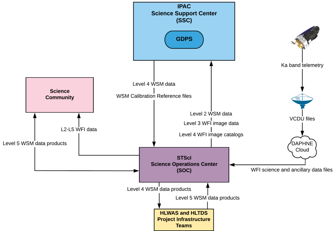
Figure 1: Operational interfaces and basic data flow for the Roman Grism-Prism Data Pipeline System (GDPS). Basic calibrated, Level-2 WFI spectroscopic data, together with Level-3 and 4 WFI image data (image and source detection catalogs) are retrieved by the SSC. Level-4 grism and prism science data products, along with calibration reference files, are delivered to the Roman archive by the SSC. The HLWAS and HLTDS Project Infrastructure Teams retrieve Level-4 Wide Field Spectroscopy Mode data products from the archive, produce Level-5 products, and return them to SOC for ingestion into the Roman archive.
