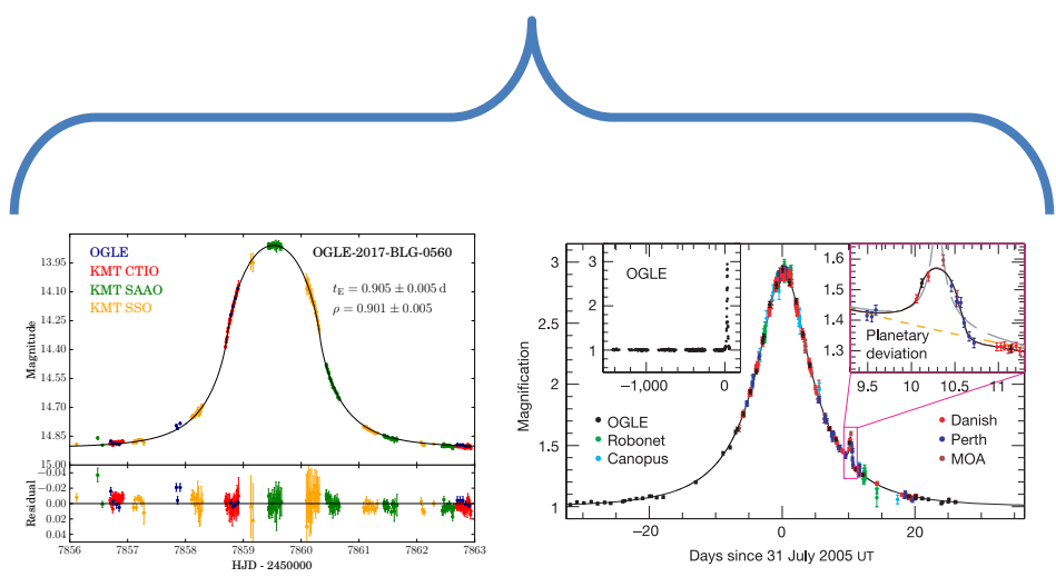
Single-lens Free-floating Planet Candidate
